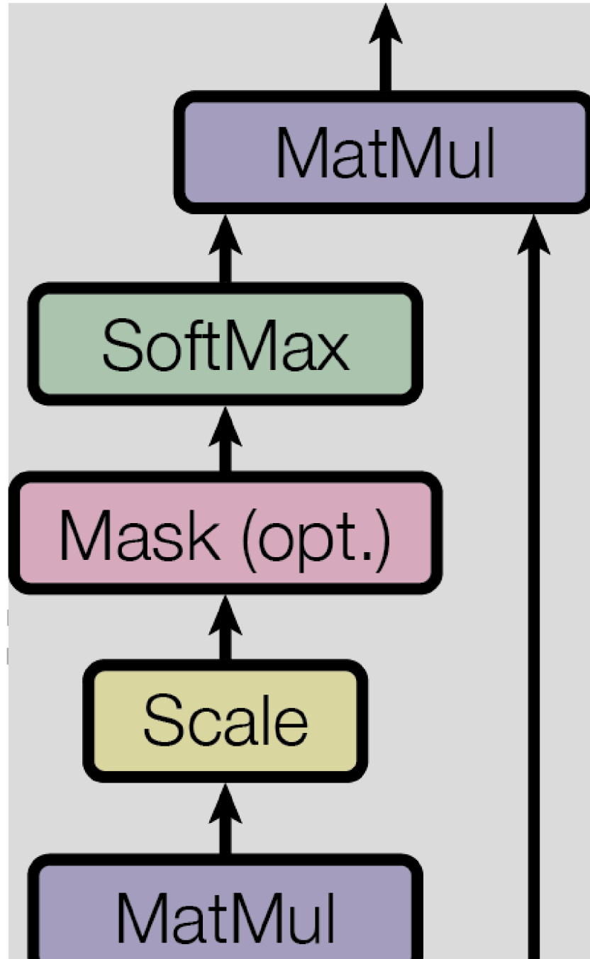
Scaled Dot-Product Attention
