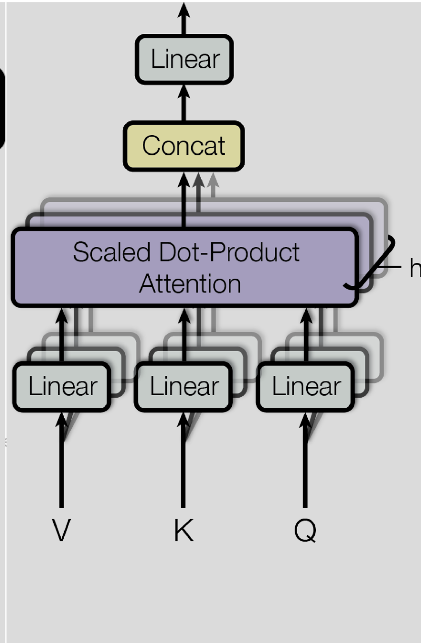
Multi-Head Attention
